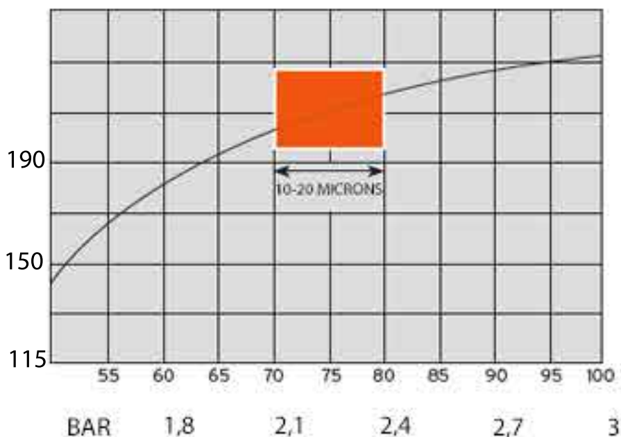
Liter/Minute 4" DESILTER CONE PERFORMANCE
